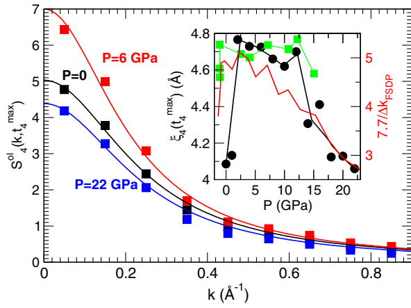
FIG. 2. Small k behavior of S_4^{\text{ol}}(k, t_4^{\text{max}}) for selected pressures in liquid NS2 at 2000 K, fitted by Eq. (2) (solid lines). The inset shows the Ornstein-Zernike fitted correlation length \xi_4 as a function of pressure for 2000 K (filled black circles) and 1500 K (filled green boxes). Right axis (red) shows the Si-O coherence length 7.7/\Delta k_{\text{FSDP}} obtained from the static structure factor [22] in the glassy state (300 K). See text for details.
