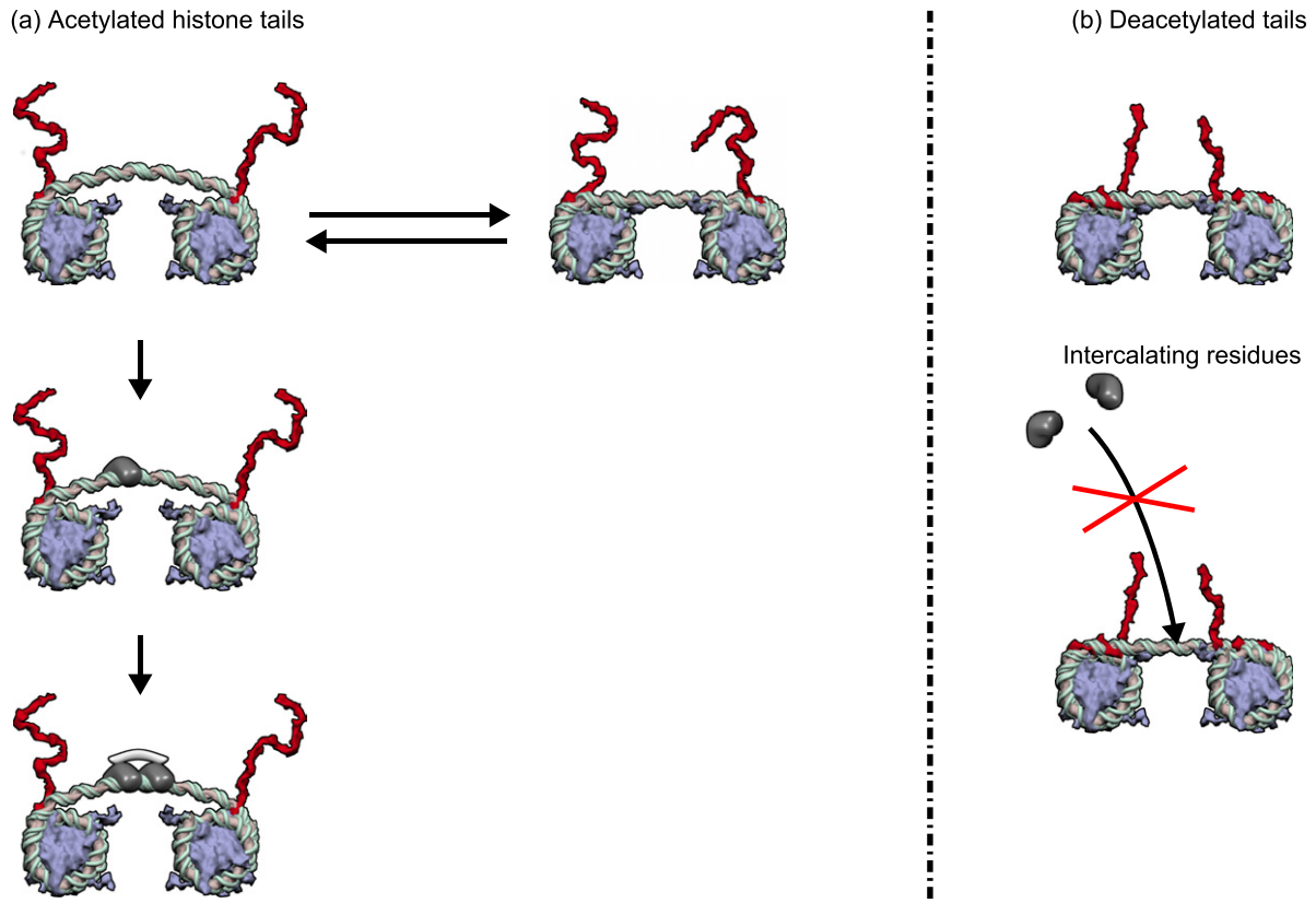
Figure 1. Epigenetically controlled DNA allostery in a chromatin fiber. H3-histone tail acetylation controls the strength of linker DNA binding onto the nucleosomes, whose orientation is fixed by their embedding in the condensed 30 nm chromatin fiber. (a) When H3 histone tails (in red) are acetylated, DNA anchoring onto nucleosomes is loose and accommodates two linker DNA conformations: a straight T-form (right), where even a single binding is barely possible and a buckled R-form (left) prone to multiple bindings. The binding of a first intercalating protein residue shifts the conformational equilibrium, in an instance of conformational capture: linker DNA buckling is stabilized and energetically favors subsequent intercalations, in a typical instance of DNA allosteric transition [67]; in particular, the binding of bis-intercalating proteins is possible [35]. (b) The tight anchoring of linker DNA onto nucleosomes in a chromatin fiber with deacetylated histone tails (in red) prevents DNA buckling transition; multiple intercalations are then energetically prohibited due to mechanical constraints [67].
