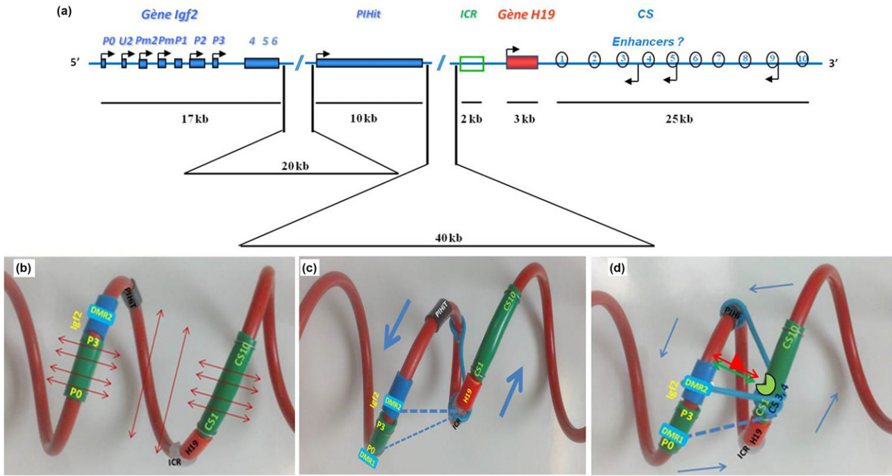
Figure 5. Chromatin fiber allostery and Igf2 gene remote activation. (a) Linear map of the mouse Igf2/H19 gene locus. Promoters of the Igf2 gene (P0-P3) are indicated by black arrows. The locus is containing two other genes named PIH1 and H19 . Remote enhancers named CS1–CS10 are located downstream of the H19 gene and about 90 kb away from the Igf2 gene. The Imprinting-Control Region (ICR), that inherits DNA methylation when paternally inherited, is located 3kb upstream of the H19 gene. (b) Folding of the Igf2/H19 locus in the context of the statistical helix. Note: even in the absence of locus specific interactions, the Igf2 promoters (P0–P3) are located close to the enhancers (CS1–CS10) in the tridimensional space. During mouse development, allele specific interactions occur, leading to different folding of the locus on the two parental chromosomes. (c) On the maternally inherited chromosome, the CTCF (CCCTC-binding Factor) insulator protein binds to the unmethylated Imprinting-Control Region (ICR) thus promoting specific interactions with other regions of the locus (blue bars) that move the enhancers away from the Igf2 promoters (blue arrows). The Igf2 gene is thus transcriptionally silent on that chromosome. (d) On the paternally inherited chromosome, DNA methylation of the ICR prevents CTCF binding and tissue-specific TFs bound to the enhancers (red triangle, green circle) thus inducing locus specific interactions (blue bars) and stabilizing the contacts between a specific enhancer, here CS4 and the Igf2 gene. Altogether, at this locus, specific interactions alter the statistical shape of the chromatin fiber in chromosome- and tissue-specific ways, depending on the DNA methylation status of the ICR and on the TFs bound on the enhancers. Such chromatin allosteric effects allow the harmonious regulation of Igf2 transcription (figure adapted from [60]).
