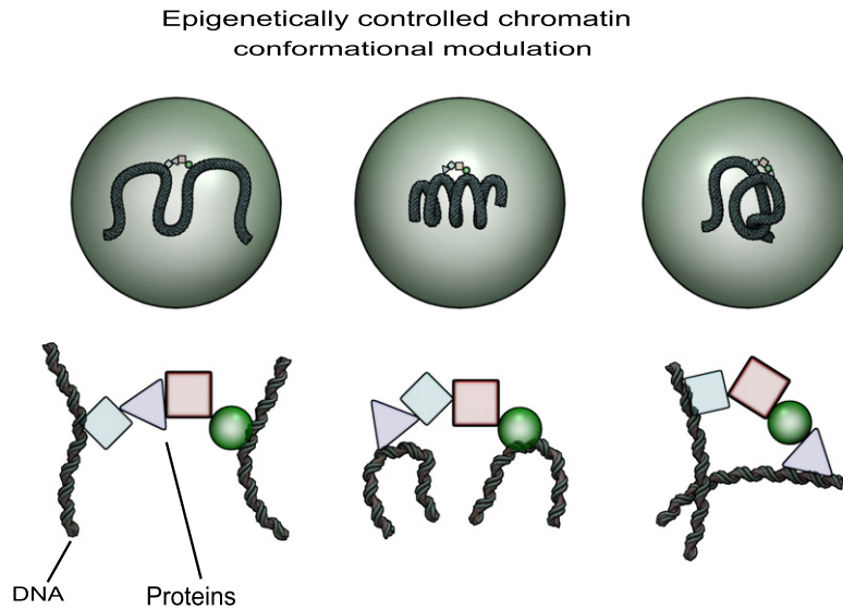
Figure 4. Chromatin conformation controls complex assembly. Physiological factors and signals, possibly epigenetically mediated, control the subset of statistically dominant chromatin fiber conformations (top, each circle correspond to a different cell state). In turn, the fiber conformation controls binding of factors to DNA and subsequent cofactor binding. Shift in the distribution of chromatin fiber conformations channels the assembly of different regulatory complexes.
