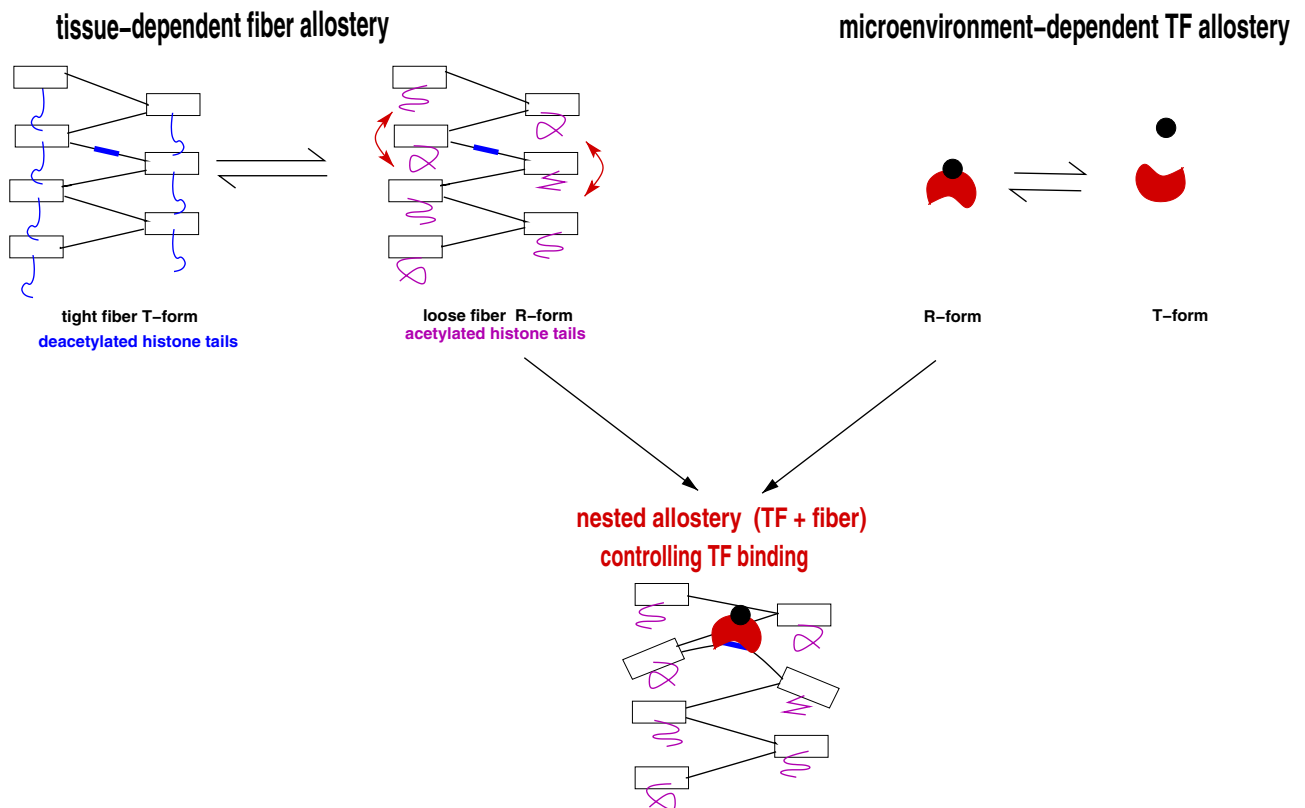
Figure 3. Nested allosteric mechanisms in eukaryote transcriptional regulation. (Top left) Histone acetylation, here H4K16ac triggers an allosteric transition of the fiber from a tight and mechanically constrained form to a loose form, namely from a T-form to R-form when using the terminology of [42]. In this transition, nucleosomes and linkers gain respectively tilting and buckling degrees of freedom. This allosteric mechanism is tissue dependent, having as effector the HATs and as active sites all the potential protein binding sites present in the embedded linker DNAs. (Top right) Molecular effectors brought in the microenvironment through signaling or metabolic pathways trigger an allosteric transition of TFs, from an inactive T-form to an R-form capable to bind to sufficiently relaxed linker DNA. (Bottom) The conjunction of the two allosteric transitions at the TF and fiber levels controls TF binding therefore participates in transcriptional regulation.
