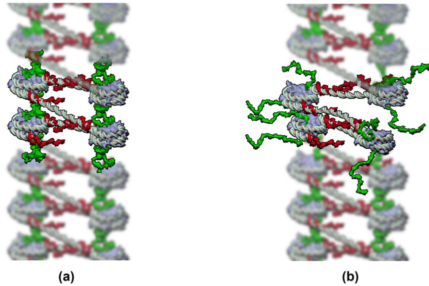
Figure 2. Effect of H4 histone tail acetylation on the chromatin fiber structure. (a) Deacetylated H4-tails (in green) protrude normally to the nucleosome core particle and ensure nucleosome stacking through tail-bridging interactions between their positively charged lysines and the acidic patches of the globular domain of the histone octamer. Deacetylated H3-tails (in red) protrude laterally near the dyad axis at the entry/exit site and constrain the anchoring of the linker DNAs on the histone octamer. (b) Acetylation of H4 histone tails weakens stacking interactions between spatially adjacent nucleosomes and allows unstacked nucleosomes to rotate, hence their flanking linker DNAs to bend despite of the anchoring constraints exerted by the deacetylated H3-tails.
