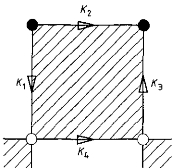
Figure 1. Unit cell of a chiral checkerboard lattice. The full circles denote spins that are decimated.
