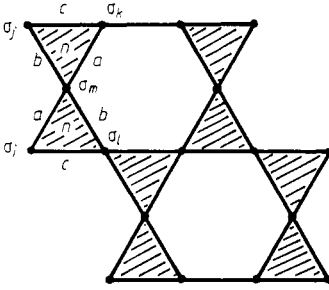
Figure 4. Potts model on a Kagomé lattice.
