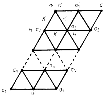
Figure 7. Ising model with a magnetic field on a triangular strip.
