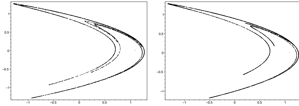
Figure 1. The attracting sets for c = 0 (left) and c = 0.1 (right)
