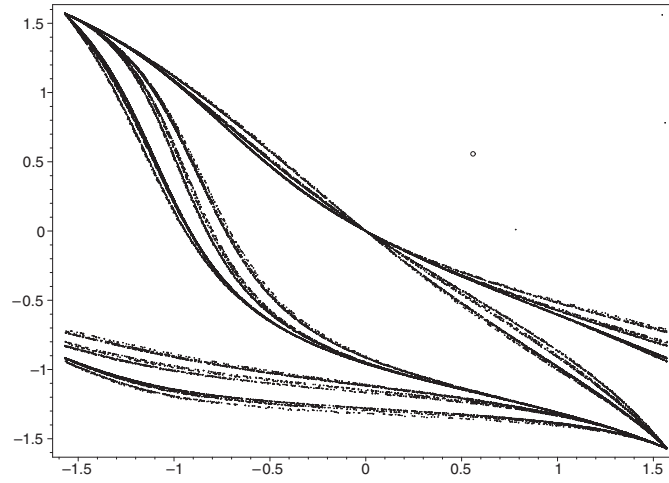
Figure 6. Phase portrait in the variables (\theta_u, \theta_v) for b = -3/5 . The open circle shows the fixed point of order 1.
