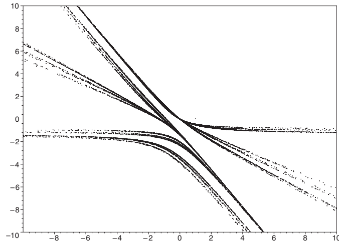
Figure 5. Phase portrait in the variables (u, v) for b = -3/5 .
